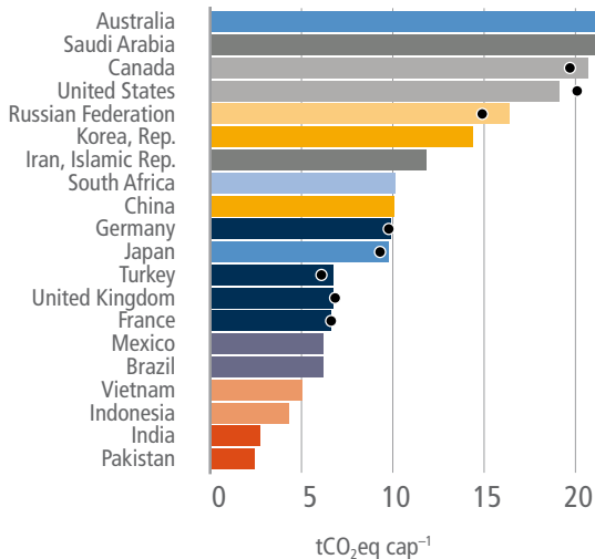
Figure 2.9 | Change in regional GHGs from multiple perspectives and their underlying drivers.
