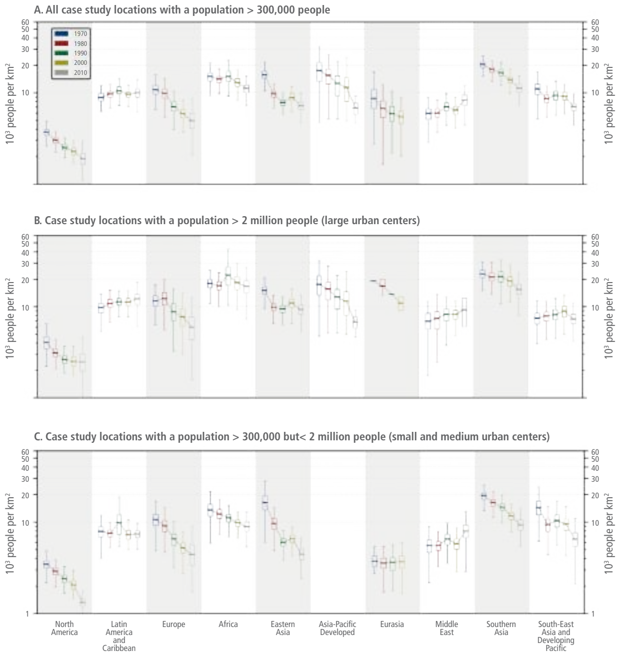
Figure 8.5: Urban population density by decade (1970–2010) grouped by the AR6 WGIII 10-region aggregation. Panel (a) displays the results from all case study locations with a population >300,000 . Panels (b) and (c) show results grouped by city size: (b) cities with a population >2 million (large urban centres), and (c) those with a population >300,000 but <2 million (small and medium urban centres). Box plots show the median, first and third quartiles, and lower and upper mild outlier thresholds of bootstrapped average urban population densities at the turn of each decade. The estimates are shown on a logarithmic scale. The data shows an overall trend of declining urban population densities among all but one region in the last four decades, at varying rates – although the Latin America and Caribbean region indicates relatively constant urban population density over time. The Middle East region is the only region to present with an increase in urban population density across all city sizes. Source: adapted from Güneralp et al. (2020).
