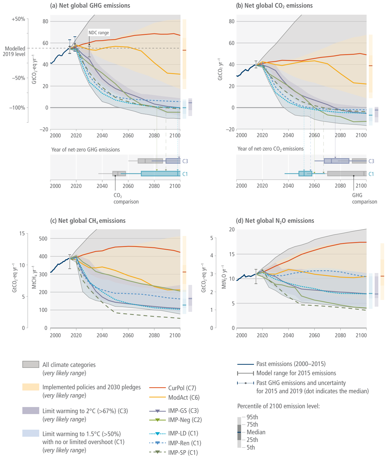
Figure TS.10 | Mitigation pathways that limit warming to 1.5°C, or 2°C, involve deep, rapid and sustained emissions reductions. Net zero CO 2 and net zero GHG emissions are possible through different mitigation portfolios.
