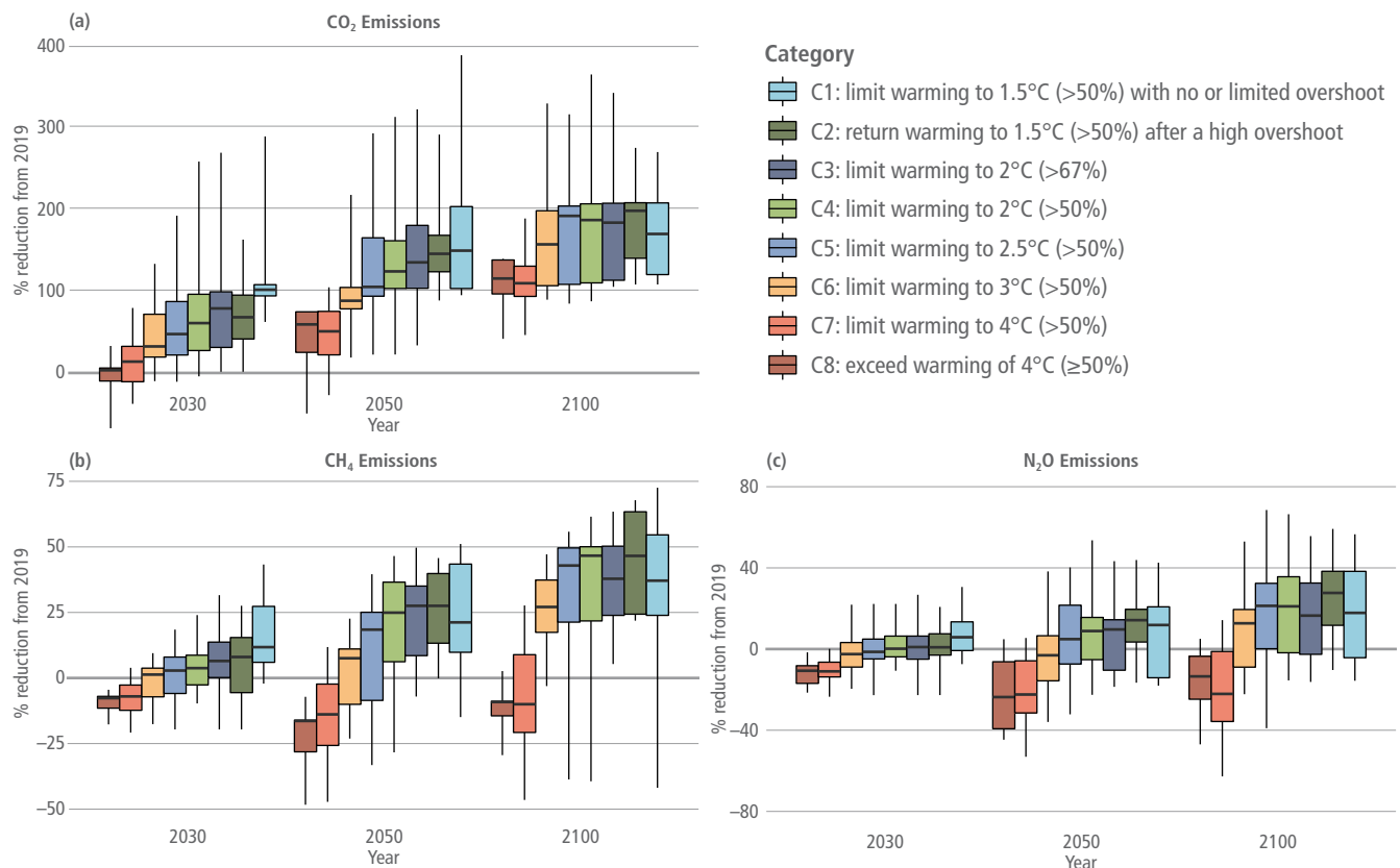
Figure 3.27 | Reduction in AFOLU GHG emissions from 2019. The AFOLU CO 2 estimates in this figure are not necessarily comparable with country GHG inventories (see Chapter 7).
