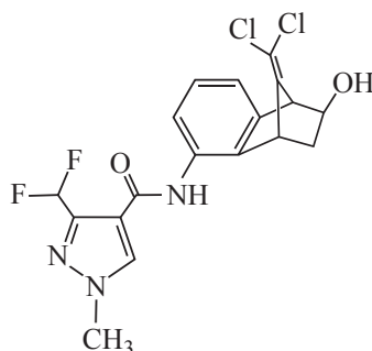
Figure 1. Chemical structure of metabolite SYN546039 (CSCD695908)
