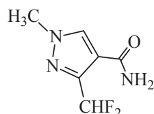
Figure 4. Chemical structure DFPA-CONH 2
