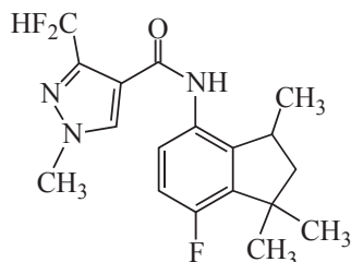
Figure 1. Chemical structure of fluindapyr (F9990/IR9792)
