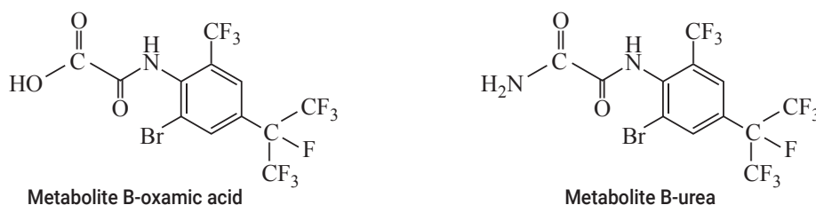
Figure 14. Chemical structures of B-oxamic acid and B-urea
