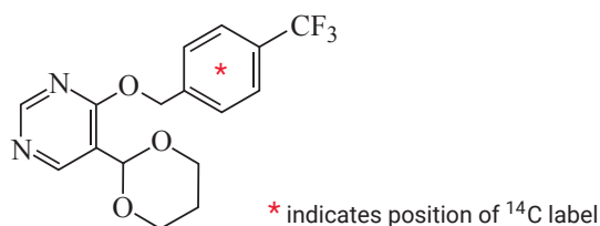
Figure 2. Position of radiolabel in phenyl-labelled benzpyrimoxan
