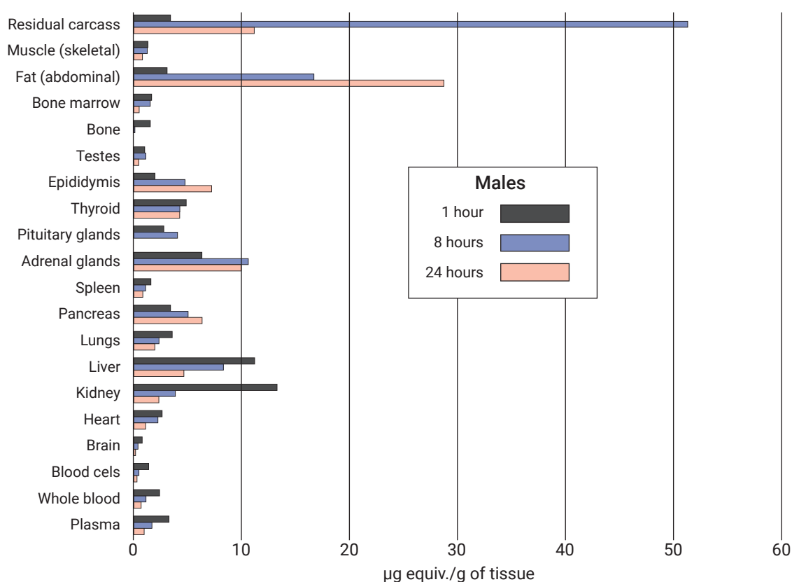
Figure 3. Mean tissue concentration of radioactivity (in mg/kg tissue) after single oral administration of [ C -ring- U - ^{14} C]broflanilide at a dose level of 500 mg/kg bw at 1, 8 and 24 hours.
