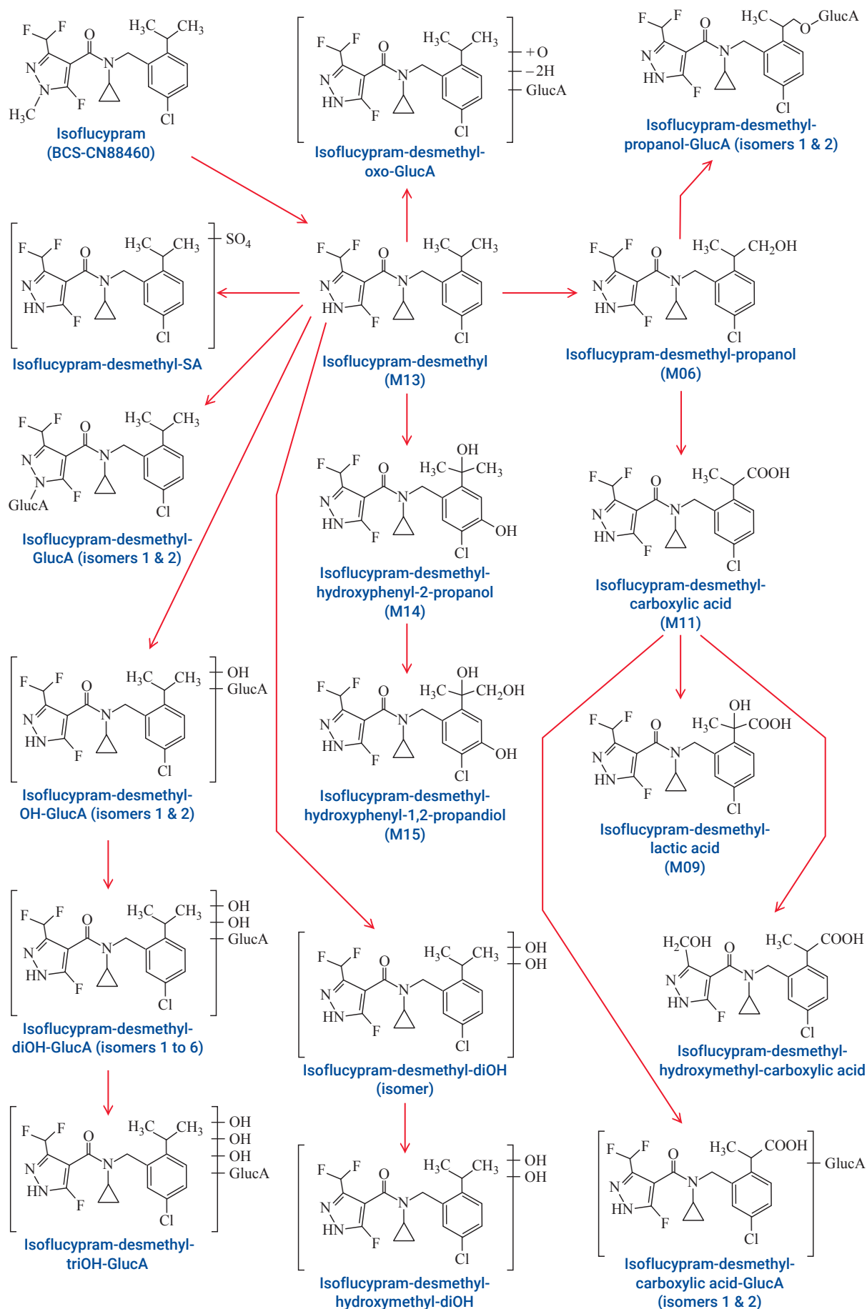
Figure 3b. Predicted metabolic pathways of isoflucypram in rats (Bongartz & Bartelsen, 2017a, b)
